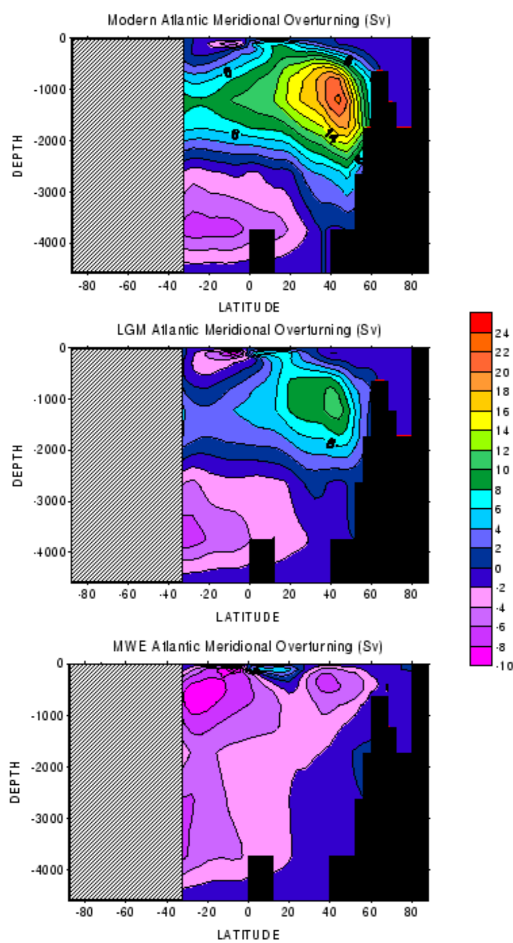
Figure 1. Meridional overturning stream function showing total transport of water in vertical plane in the Atlantic Ocean. From top to bottom: present-day overturning, LGM, and MWE. Transport in Sv ( 1 \text{ Sv} = 10^6 \text{ m}^3/\text{s} ).
