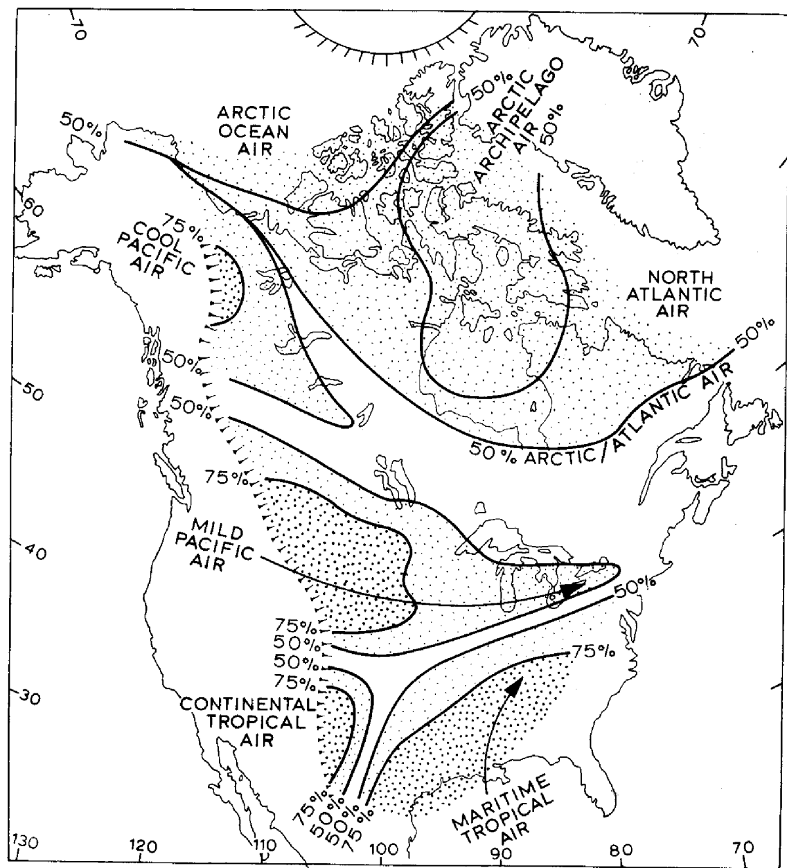
Fig. 5.13. Regions in North America east of the Rocky Mountains dominated by the various air-mass types in July for more than 50% and 75% of the time (after Bryson 1966). The 50% frequency lines correspond to mean frontal positions.
