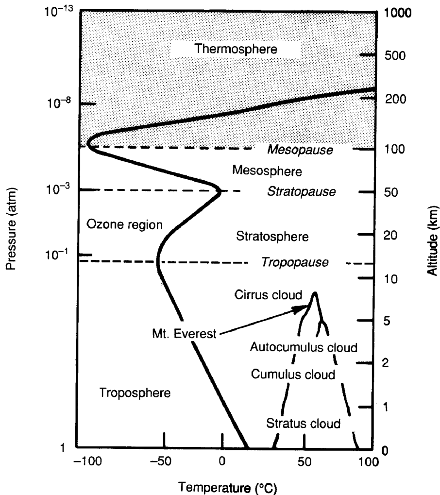
Figure 3.5 The variation of atmospheric pressure and temperature with altitude above Earth's surface. Typical heights of a few cloud types are indicated. (Adapted with permission from W. L. Chameides and D. D. Davis, Chemistry in the troposphere , Chemical and Engineering News , 60 (40), 38–52. Copyright 1982 by the American Chemical Society.)
