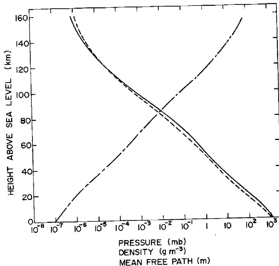
Fig. 1.4 Vertical profile of pressure in millibars (---), density in grams per cubic meter (—), and mean free path in meters (— · —) for U.S. Extension to International Civil Aviation Organization Standard Atmosphere. (Adapted from "CRC Handbook of Chemistry and Physics," 54th Edition, © CRC Press, Cleveland, 1973, pp. F186–190. Used by permission of CRC Press, Inc.)
