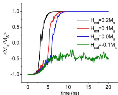
FIG. 5. (Color online) The magnetization dynamics in current density of 9.0 \times 10^7 \text{ A/cm}^2 under different external fields.
