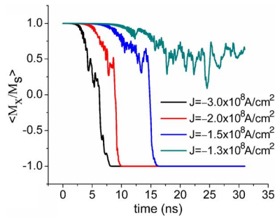
FIG. 4. (Color online) The temporal evolution of the x component of magnetization M_x under four different current densities.
