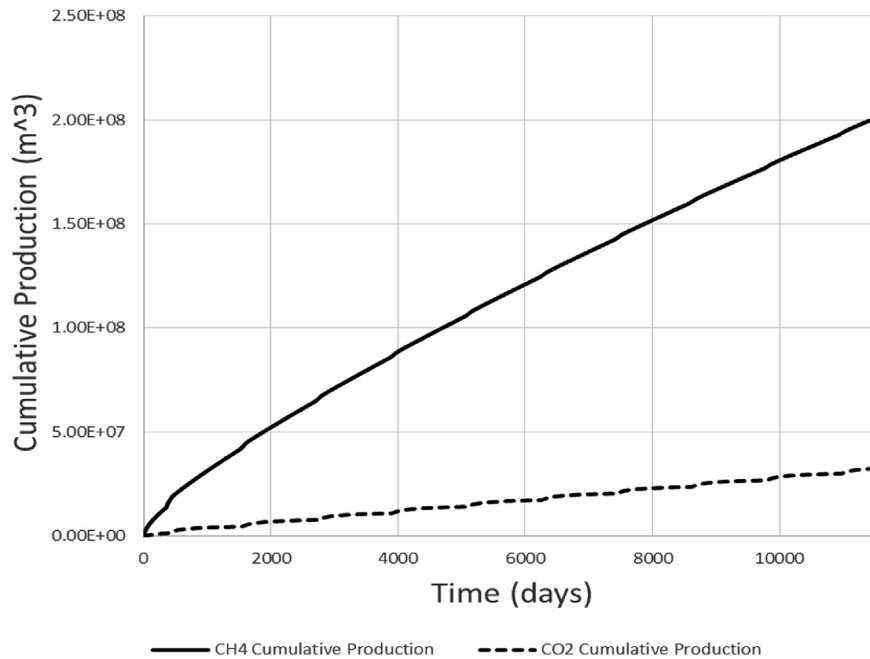
Fig. 14. Cumulative production of CH_4 (solid line) and CO_2 (dash line) under optimal pulsed injection.
